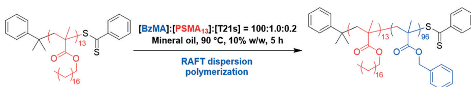
Scheme 1. Synthesis of poly(stearyl methacrylate) 13 -poly(benzyl methacrylate) 96 (PSMA 13 -PBzMA 96 ) vesicles via RAFT dispersion polymerization of benzyl methacrylate at 10% w/w solids in mineral oil at 90 °C.
