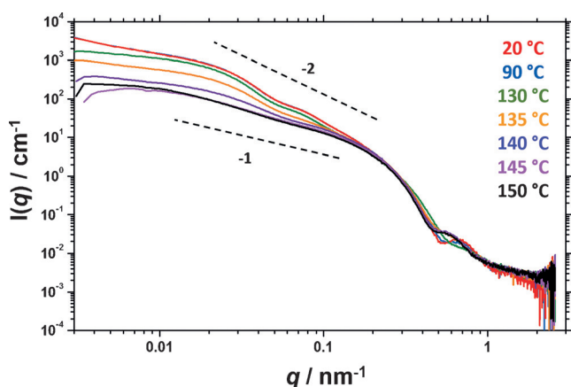
Figure 2. Variable temperature small-angle X-ray scattering (SAXS) patterns recorded for a 5.0% w/w dispersion of PSMA 13 -PBzMA 96 nano-objects in mineral oil. Gradients of -2 and -1 are shown as a guide to the eye.
