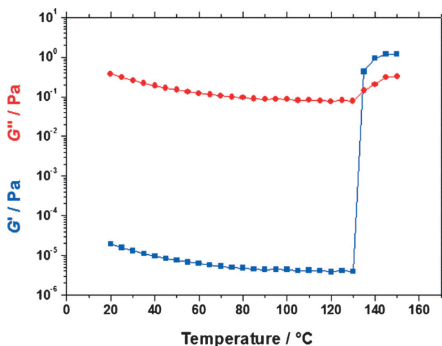
Figure 5. Dependence of the storage modulus ( G' , blue data) and loss modulus ( G'' , red data) of a 10% w/w dispersion of PSMA 13 -PBzMA 96 nanoparticles in mineral oil upon heating from 20 to 150 °C. Data were obtained at 1.0% strain using an angular frequency of 10 rad s -1 , with a heating rate of 2 °C min -1 .
