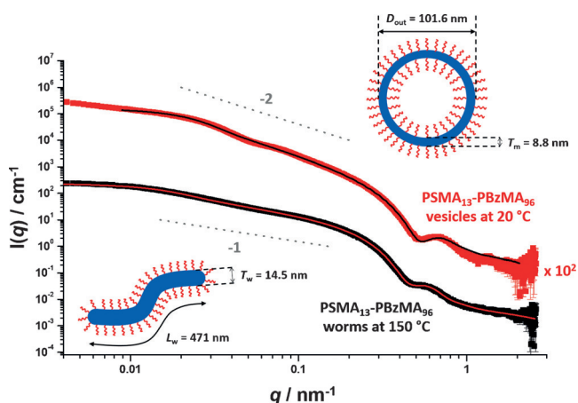
Figure 3. Representative SAXS patterns and fittings for PSMA 13 -PBzMA 96 vesicles at 20 °C (top, red data set plus black data fit) and PSMA 13 -PBzMA 96 worms at 150 °C (bottom, black data set plus red data fit). Inset cartoons indicate the mean overall vesicle diameter ( D_{out} ), vesicle membrane thickness ( T_m ), worm contour length ( L_w ) and worm thickness ( T_w ). Gradients of -2 and -1 are also shown as a guide to the eye.
