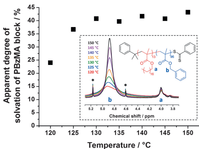
Figure 4. Temperature dependence of the apparent degree of solvation of PBzMA block as judged by variable temperature 1 H NMR studies of a 5.0% w/w PSMA 13 -PBzMA 96 nanoparticles in d 26 -dodecane (see inset for assigned partial spectra from which these degrees of solvation were determined). Asterisks indicate satellite signals.
