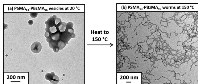
Figure 1. Transmission electron micrographs obtained for a) 0.1% w/w PSMA 13 -PBzMA 96 vesicles at 20 °C and b) the highly anisotropic worms formed by the same vesicle dispersion on heating up to 150 °C.
