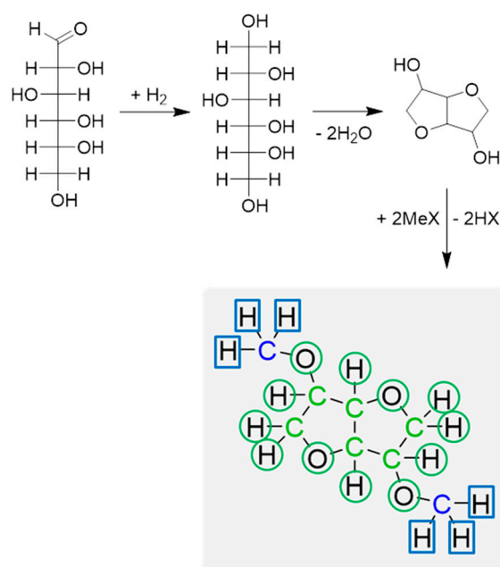
Figure 2. A scheme of a dimethyl isosorbide synthesis, producing a product with 75% bio-based carbon content and 83% total bio-based content. Green atoms are known to be bio-based from direct analysis; blue atoms are known to be not bio-based from analysis; atoms in green circles are assigned to be bio-based; atoms in blue circles are assigned not to be bio-based.
