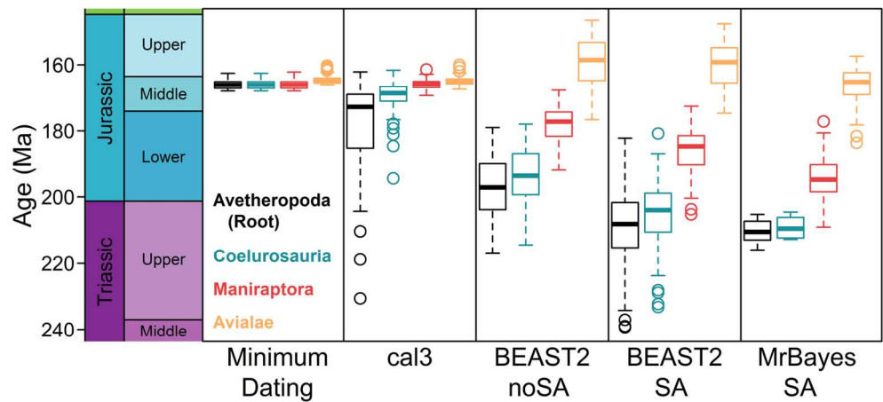
Figure 1. Age estimates for four nested theropod clades, across five different approaches for obtaining a dated phylogeny using the Xu et al. [1] dataset. 69x32mm (600 x 600 DPI)
