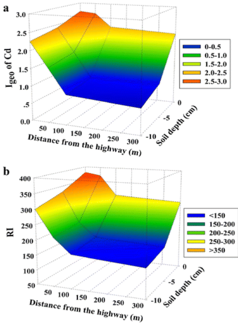
Fig. 3: The 3D response surface of the I_{geo} of Cd (a) and RI of heavy metal (b)
