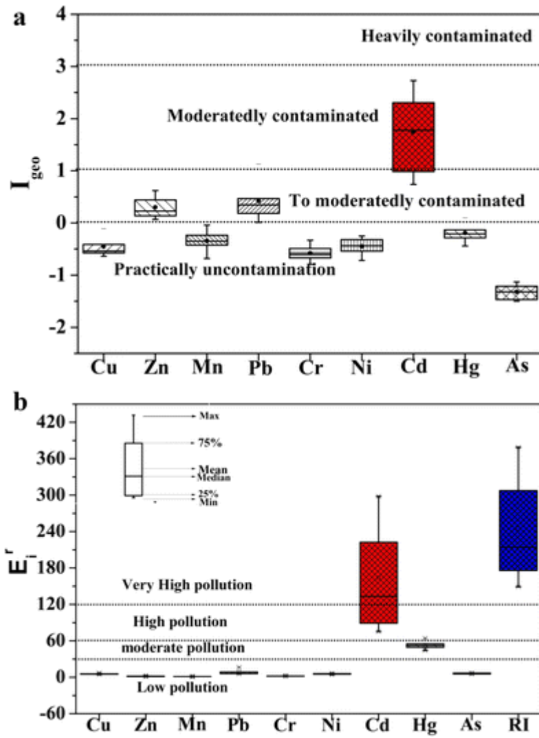
Fig 2: The geo-accumulation index ( I_{geo} ) (a) and the total potential ecological risk (RI), monomial potential ecological risk index ( E_i' ) (b) for Cu, Zn, Mn, Pb, Cr, Ni, Cd, Hg, and As in soil samples collected along the 108th National Highway
