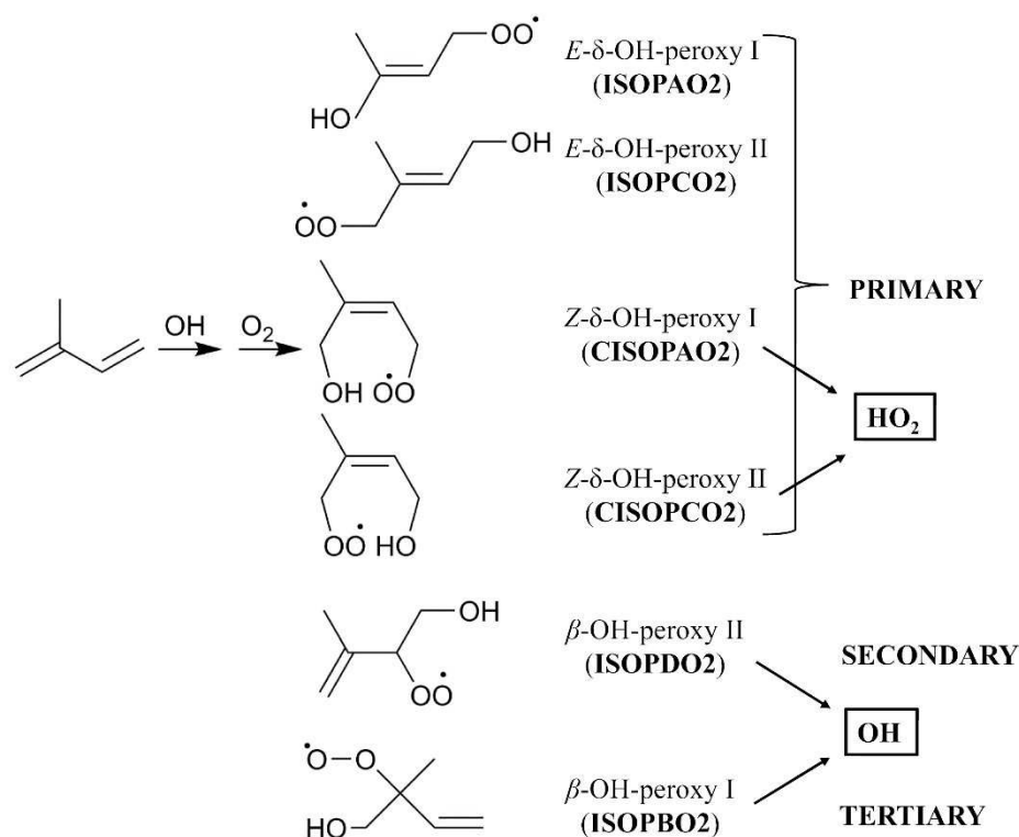
Figure 6. Isomers of HO-Iso- \text{O}_2 , after Peeters et al. 30 The nomenclature in bold type within parentheses corresponds to that used in the MCM v 3.3.1. 56 Isomers are classified according
