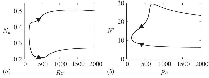
Figure 1. Bifurcation diagram showing the lower (downward triangle) and upper (upward triangle) branches of ECS as a function of the Reynolds number Re in terms of (a) N_u = \int_D u_0^2 dy dz / \int_D dy dz , (b) N' = \int_D (v_1^2 + w_1^2) dy dz / \int_D dy dz . The branches are connected via a saddle-node bifurcation at Re \approx 136 . Lower branch states are computed on a 32 \times 64 mesh while upper branch states are computed on a 64 \times 128 mesh.
