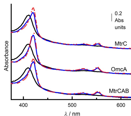
Figure 7. Photoreduction of MtrC, OmcA, and MtrCAB solutions by RuP-TiO 2 -MtrC particles. Electronic absorbance of RuP-TiO 2 -MtrC suspensions (0.037 mg mL -1 ) with 0.65 \mu M MtrC (top), 0.61 \mu M OmcA (middle), and 0.31 \mu M MtrCAB (bottom) before (black) and after (blue) 30 min illumination ( \lambda > 390 nm, power \approx 400 W m -2 ), followed by the addition of excess sodium dithionite (red). Experiments performed at 20 °C in anaerobic 150 mM MES (pH 6) with Triton X-100 (0.2%, v/v) included for MtrCAB. Spectra offset on the y-axis for clarity.
