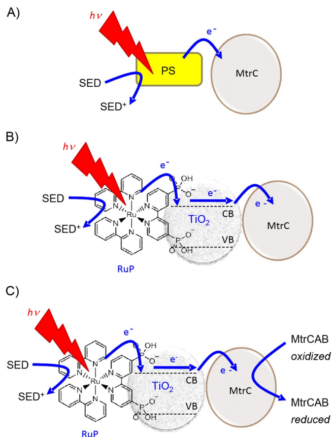
Figure 2. Schematic representation of strategies for photoreduction of MR-1 cytochromes investigated in this work, illustrated for MtrC and MtrCAB. A) Photoreduction of MtrC by a soluble photosensitizer (PS), which may be an organic dye or an inorganic complex. B) Photoreduction of MtrC adsorbed on TiO 2 nanoparticles sensitized with a phosphonated Ru II dye (RuP). C) Photocatalytic reduction of solutions of MtrCAB by MtrC-coated, dye-sensitized TiO 2 particles. SED: sacrificial electron donor. CB: conduction band. VB: valence band.
