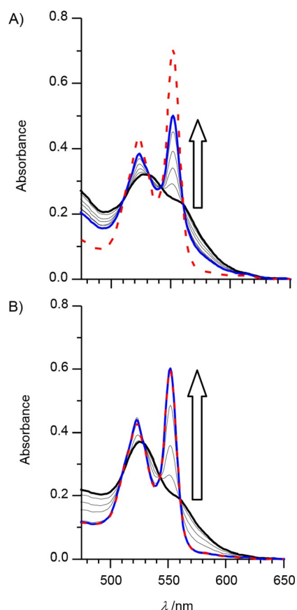
Figure 3. Photoreduction of MtrC by A) FMN, and B) eosin Y, visualized by electronic absorbance spectroscopy. A) Spectra of an MtrC (32 \mu\text{M} )/FMN (10 \mu\text{M} ) solution as prepared (black line) and after illumination for 5, 15, 30, 60, 90 (gray lines), and 120 min (blue line) prior to the addition of excess dithionite (dashed red line). B) Spectra of an MtrC (26 \mu\text{M} )/eosin Y (14 \mu\text{M} ) solution as prepared (black line) and after illumination for 5, 15, 30, 60 (gray lines), and 90 min (blue line) prior to the addition of excess dithionite (dashed red line). Arrows indicate the direction of spectral change during illumination ( \lambda > 390 nm, power \approx 400 W m -2 ). Anaerobic samples in 50 mM TEOA, 50 mM HEPES, 2 mM CaCl 2 , 10 mM KCl, pH 7 at 20 °C. Path length: 1 mm.
