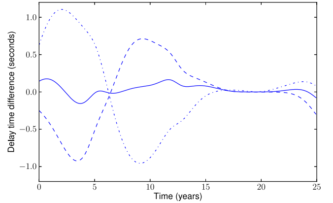
Figure 1. The difference in the planet-induced LTT delays of Keplerian versus Newtonian models for a typical two-planet fit for NN Ser. Three cases are shown: astrometric (dashed–dotted), Jacobi (dashed) and modified Jacobi (solid). The MJD = 54500 reference time corresponds to the time around 19 yr in when all models agree. For reference the LTT variations in NN Ser have a range of \pm 40 s. The Newtonian comparison orbits are calculated separately for each of the three coordinate systems.
