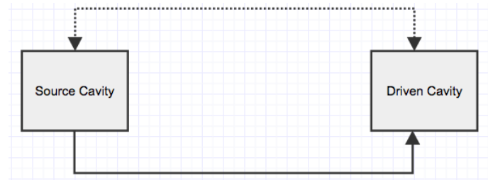
FIG. 7: Schematic plot of the feedback loop between the two cavities. We envision a scenario of two coupled cavities; a source cavity and a driven cavity. The driven cavity is assumed to be slaved to the source cavity. The source cavity drives the state of the slave cavity by means of a unidirectional coupling (shown by a solid line). The driven cavity in turn also influences the state of the source cavity by means of a reversible interaction (shown by a dotted line). The simultaneous presence of reversible and irreversible couplings between the cavity modes results in an all-optical feedback loop.
