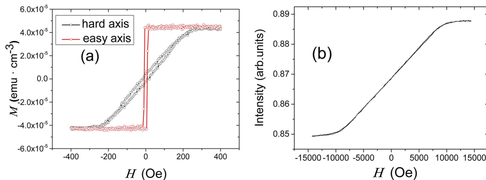
FIG. 1. (a) In-plane M-H loops along both the EA (easy axis) and HA (hard axis) for the CoFeB film deposited on GaAs(100) substrates by VSM measurement. M and H represent the magnetic moment and applied magnetic field, respectively. Figure (b) shows the Polar MOKE loop for the out-of-plane direction of the CoFeB film.
