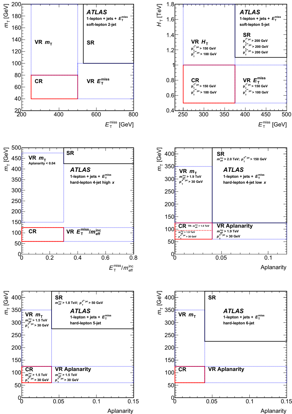
Fig. 2 Graphical illustration of the soft-lepton 2-jet (top left), soft-lepton 5-jet (top right), hard-lepton 4-jet high- x (middle left), 4-jet low- x (middle right), 5-jet (bottom left) and 6-jet (bottom right) signal (SR), control (CR) and validation (VR) regions. In addition to the two variables shown on the x and y axes, labels indicate other event selec-
