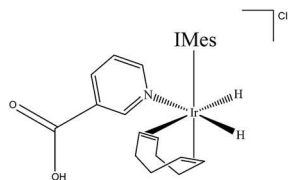
Scheme 2 [\text{Ir}(\text{H})_2(\text{COD})(\text{IMes})(\text{NA}_\text{B})\text{Cl}] ( 3a ), major product formed by \text{H}_2 addition to 2a in methanol- d_4 solution.
