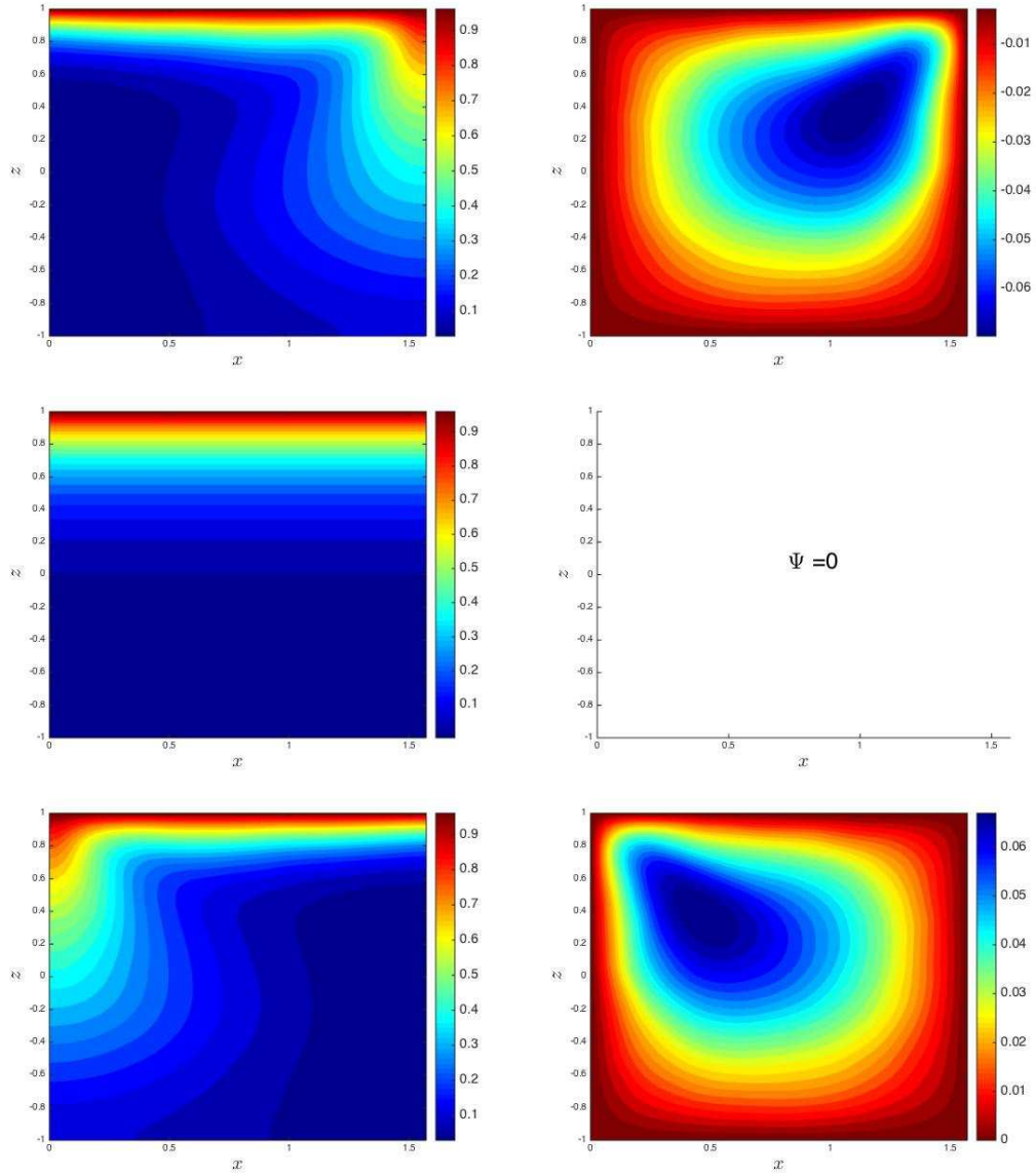
Figure 4: Example of three different solutions of problem (9) for a given heterogeneous permeability field (the left hand field in Figure 3) with parameters: Ra = 60 , Da = 0.1 , \beta_L = \pi/2 and \beta_T = \beta_L/10 . The upper branch solution is shown in the top row of figures, the trivial solution is shown in the middle row and lower branch solution is shown in the bottom row.
