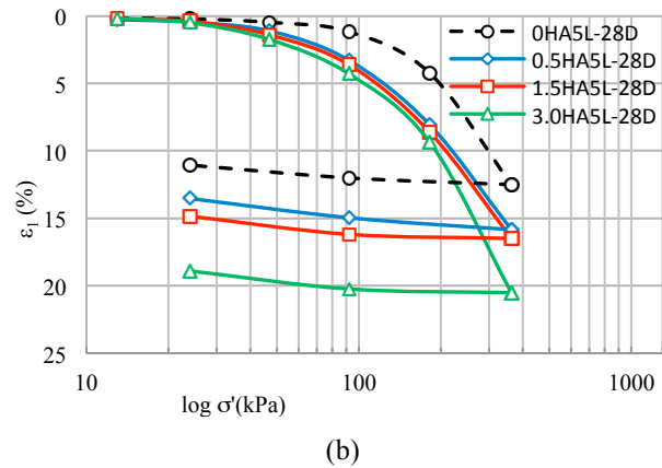
Fig. 5. Effect of humic acid on compression curves of lime-treated clay after 28 curing days, (a) e vs. \log \sigma' , (b) \epsilon_1 vs. \log \sigma' .
