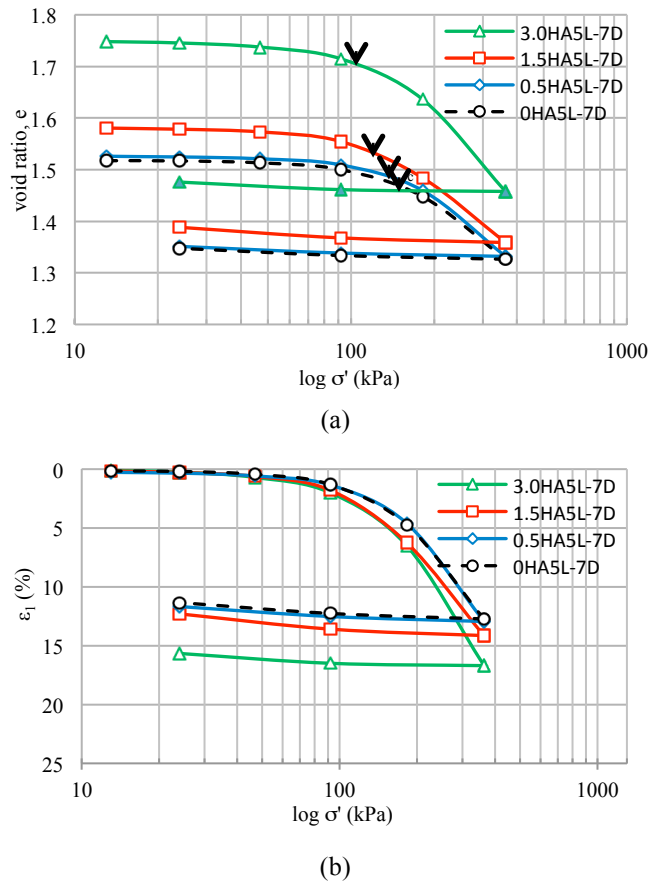
Fig. 4. Effect of humic acid on compression curves of lime-treated clay after 7 curing days, (a) e vs. \log \sigma' , (b) \varepsilon_1 vs. \log \sigma' .
