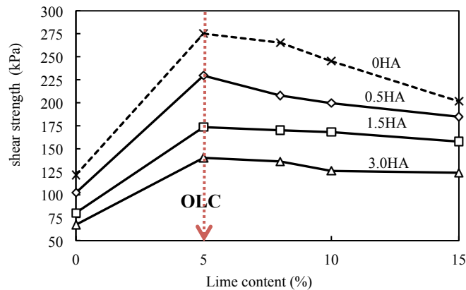
Fig. 2. Effect of lime content on the shear strength of clay with different humic acid contents after 7 days curing.
