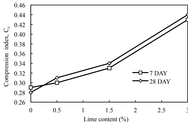
Fig. 6. Effect of compression index ( C_c ) of lime-treated clay with various humic acid content at 7 and 28 days.
