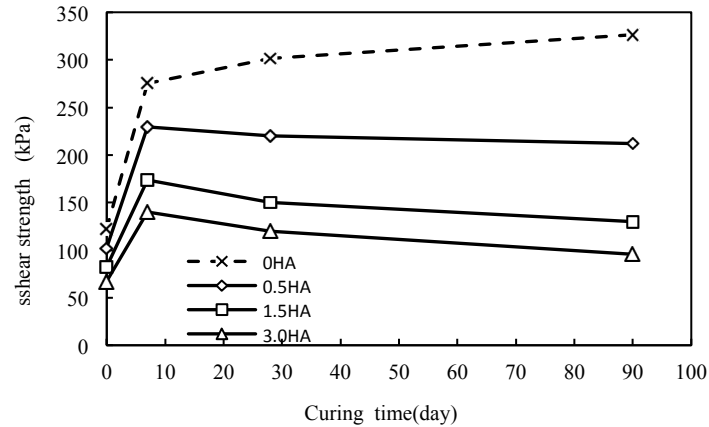
Fig. 3. Effect of curing period on the shear strength of lime-treated clay.
