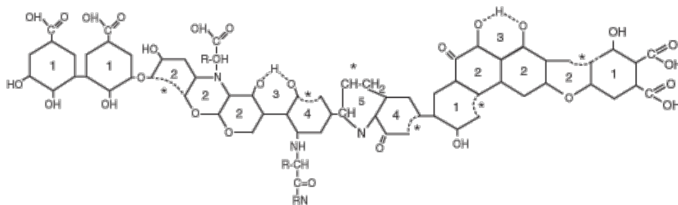
Fig. 1. The organic structure of humic acid
