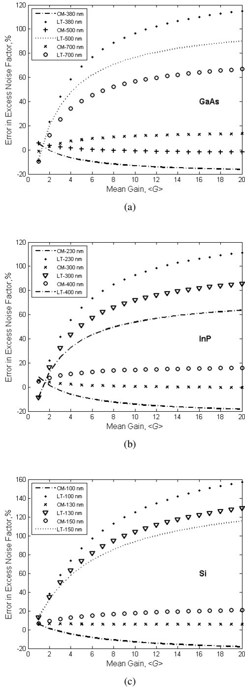
Fig. 7: Relative errors in the excess noise calculated from McIntyre's local-theory (LT) model ( k \neq 1 ) and the CM technique, as compared to ENM technique for three different widths of (a) GaAs, (b) InP and (c) Si [14]. As the gain increases, the relative error associated with the CM technique approaches a constant value.
