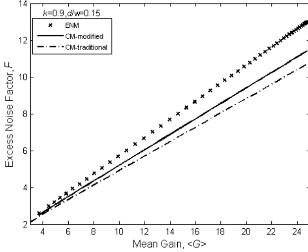
Fig. 4: The excess noise factor as a function of the mean gain is shown for the ENM and traditional CM [13] method for k=0.9 and compared to the modified CM ( k=1 ). The normalized dead space, d' , is taken to be 0.15. It can be seen that the modified CM gives a better approximation than the traditional method.
