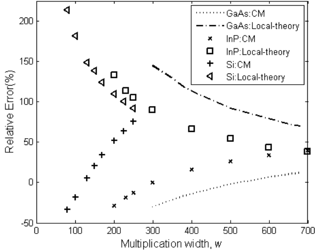
Fig. 6: Relative errors between the excess noise factors, found by comparing the ENM to McIntyre’s local-theory model (with k \neq 1 ) and the CM technique, are shown. The errors are plotted as a function of various multiplication widths of GaAs, InP and Si APD devices for a mean gain of 22. We use these values to determine the multiplication widths for which the CM approximation may be used practically.
