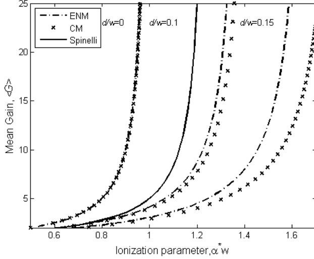
Fig. 2: Mean gain, found from ENM and CM techniques, is shown as a function of the ionization parameter, \alpha^* w , for d' = 0, 0.1 and 0.15 . These results hold for any avalanche region for which the assumption, k = 1 is justified. The mean gain found from Spinelli analytical formulation is also shown for the case of d' = 0.1 for comparison.
