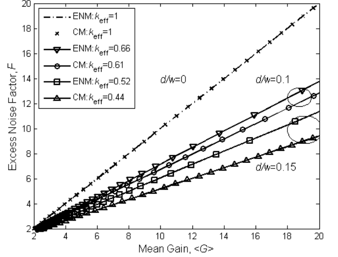
Fig. 3: The excess noise factor, F , as a function of the mean gain, \langle G \rangle , is shown for both the ENM and CM techniques. The normalized dead spaces of d' = 0, 0.1 and 0.15 are considered for comparison and the effective McIntyre ionization coefficient, k_{\text{eff}} is noted for each case and stated in the legend.
