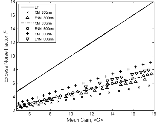
Fig. 5: The excess noise factor, F , shown as a function of the mean gain for various multiplication widths of GaAs. The CM technique predicts the excess noise far better than McIntyre's local-theory (LT) model with equal ionization coefficients assumption.
