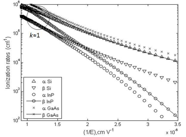
Fig. 1: The enabled ionization parameters, \alpha^* and \beta^* , as a function of the applied electric field for Si, InP and GaAs [14]. The encircled area highlights the ionization coefficients and electric field across the APD devices where the assumption k \approx 1 is valid. As an example, for a GaAs APD with the multiplication width = 0.05-0.1 \mu\text{m} [4], which has k = 0.86 and mean gain = 8, the assumption of k \approx 1 may be used to get an estimation of the mean gain and the excess noise.
