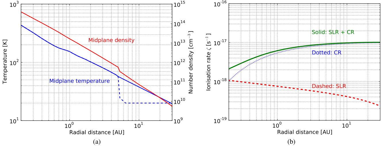
Fig. 1. a) Temperature T(R) in K (blue) and number density n(R) in \text{cm}^{-3} (red) profiles for the disk midplane. The solid blue line indicates the adjusted temperature profile (as described in the text). The original temperature profile from Alibert et al. (2013) beyond 5.2 AU is indicated by the dashed blue line. b) Ionisation rate \zeta(R) in \text{s}^{-1} adopted for the disk midplane. The red dashed line depicts the contribution to the ionisation rate from short-lived radionuclides (SLRs) only. The blue dotted line is the contribution from external cosmic rays (CRs) only. The solid green line represents the total ionisation rate (SLRs and CRs) as a function of radial distance.
