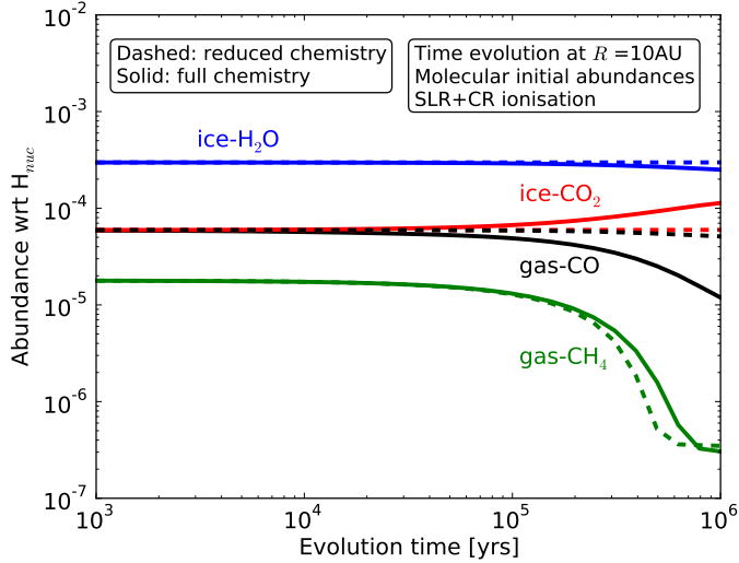
Fig. 4. Abundance evolution with time for CO gas, CO 2 ice, H 2 O ice and CH 4 gas. Dashed curves are for the reduced chemistry, solid curves are for the full chemistry. Additional time-dependent plots are supplied in Appendix A.
