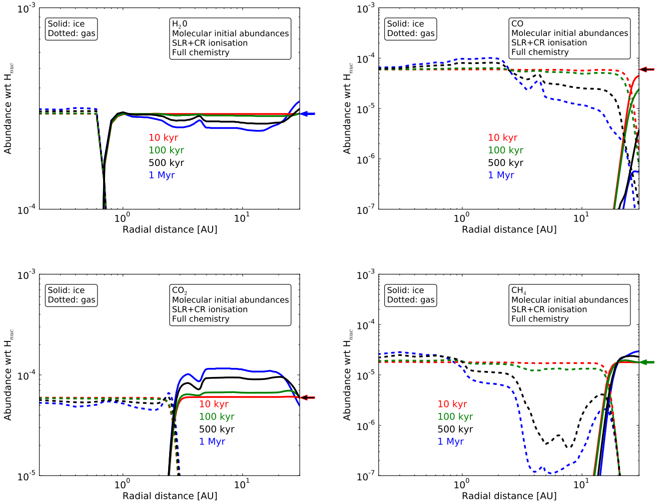
Fig. A.1. Abundances as function of radial distance R of the four key volatiles, taken at four different evolutionary stages. Note the different y -axes ranges. Arrows to the right of each panel indicate the initial abundance level in the case of the inheritance-scenario.
