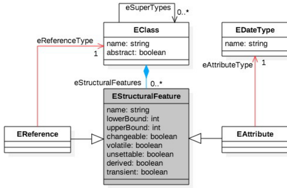
Fig. 1. The core elements of Ecore meta-model adapted from [12]
