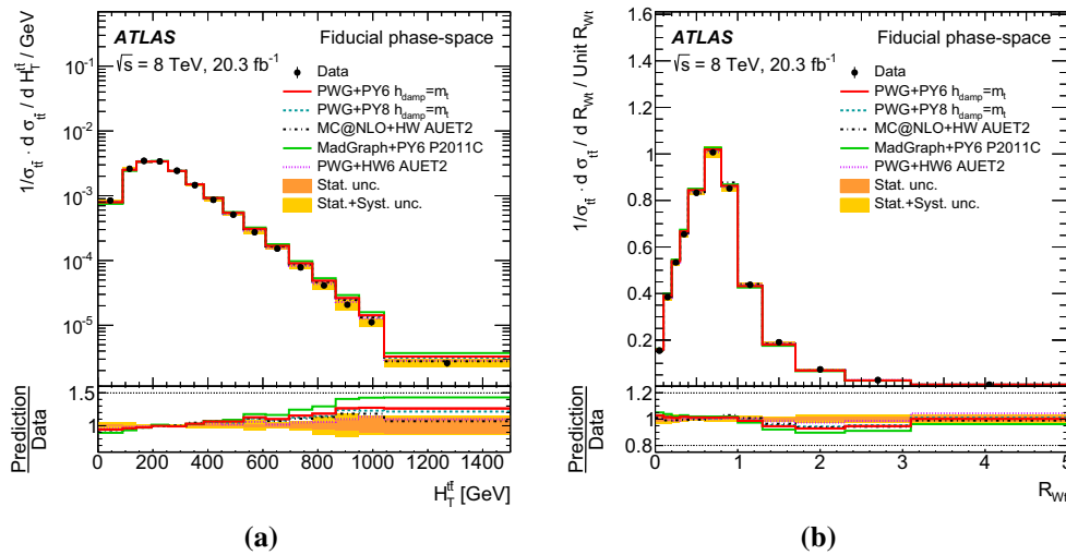
Fig. 9 Fiducial phase-space normalized differential cross-sections as a function of the a scalar sum of the transverse momenta of the hadronic and leptonic top quarks ( H_T^{fit} ) and b the ratio of the hadronic W and the hadronic top transverse momenta ( R_{Wt} ). The yellow bands indicate
