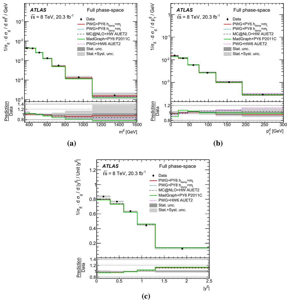
Fig. 12 Full phase-space normalized differential cross-sections as a function of the a invariant mass ( m^l ), b transverse momentum ( p_T^l ) and c absolute value of the rapidity ( |y^l| ) of the t\bar{t} system. The
