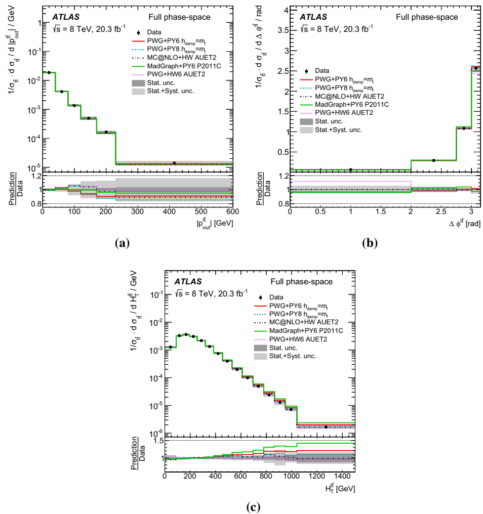
Fig. 14 Full phase-space normalized differential cross-sections as a function of the a out-of-plane momentum ( |p_{\text{out}}^{t\bar{t}}| ), b azimuthal angle ( \Delta\phi^{t\bar{t}} ), and c scalar sum of the transverse momenta of the hadronic and leptonic top quarks ( H_T^{t\bar{t}} ) of the t\bar{t} system. The grey bands indicate the total uncertainty on the data in each bin. The POWHEG+PYTHIA generator with h_{\text{damp}} = m_t and the CT10nlo PDF is used as the nominal prediction to correct for detector effects
