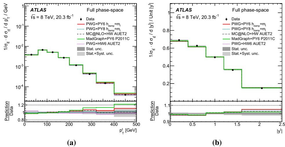
Fig. 11 Full phase-space normalized differential cross-sections as a function of the a transverse momentum ( p_T^l ) and b the absolute value of the rapidity ( |y^l| ) of the top quark. The grey bands indicate the total
