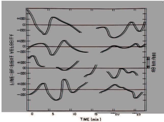
Fig. 4 Temporal variation of Doppler velocities in H-line of Ca II from Pasachoff et al. (1968).
