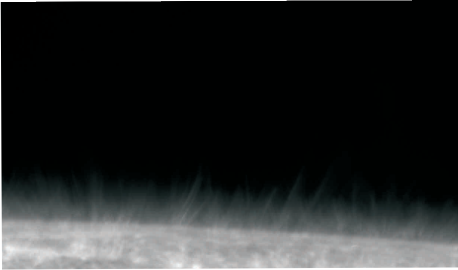
Fig. 1 High resolution image of spicules at the solar limb in Ca II H line taken by Solar Optical Telescope (SOT) on board of Hinode spacecraft (November 22, 2006).
