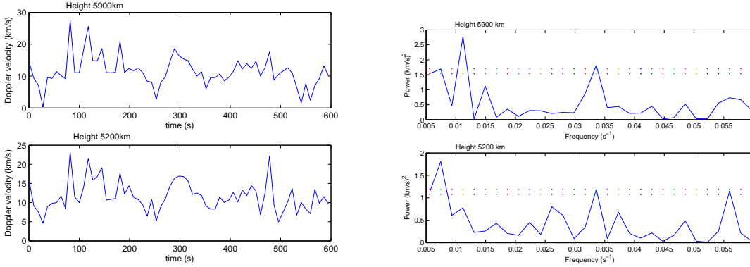
Fig. 11 Left: Doppler velocity time series at the heights of 5200 and 5900 km in one of the spicules, adapted from Zaqarashvili et al. (2007). The time interval between consecutive measurements is \sim 8 s. Right: power spectra of Doppler velocity oscillations from the time series. The dotted lines in both plots show 95.5% and 98% confidence levels, respectively. There is the clear evidence of oscillations with periods of 180 and 30 s at both heights.
