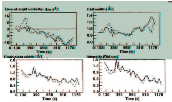
Fig. 8 Temporal variations of H\alpha line profile parameters and the line-of-sight velocity of spicules at different heights, adapted from Pampushev and Salakhutdinov (1994). The solid line corresponds to the height of 5 Mm and the dashed line to 8 Mm above the solar limb, respectively.
