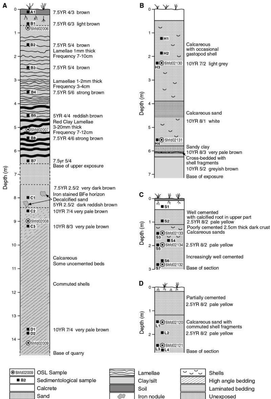
Fig. 5. Composite stratigraphy of sediments revealed through (A) Wilderness seaward cordon, (B) Hoe Walle Cliff, (C) Soetendals Valley ridge, and (D) Agulhas ridge.
