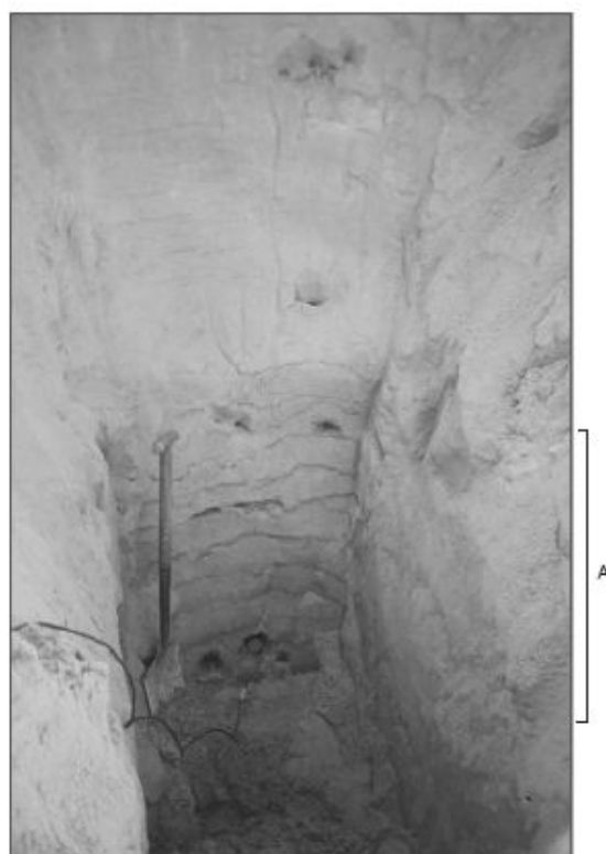
Fig. 4. Exposure of friable unconsolidated upper sand unit with (A) silty clay lamellae at the Wilderness seaward cordon.
