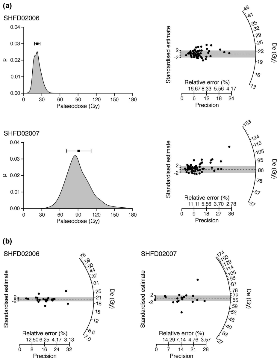
Fig. 8. OSL palaeodose data for samples Shfd02006 and Shfd02007 from Wilderness seaward cordon. (a) Single grain data plotted as probability density with the weighted mean and standard deviation above and as radial graphs, and (b) single aliquot data plotted as radial graphs.
