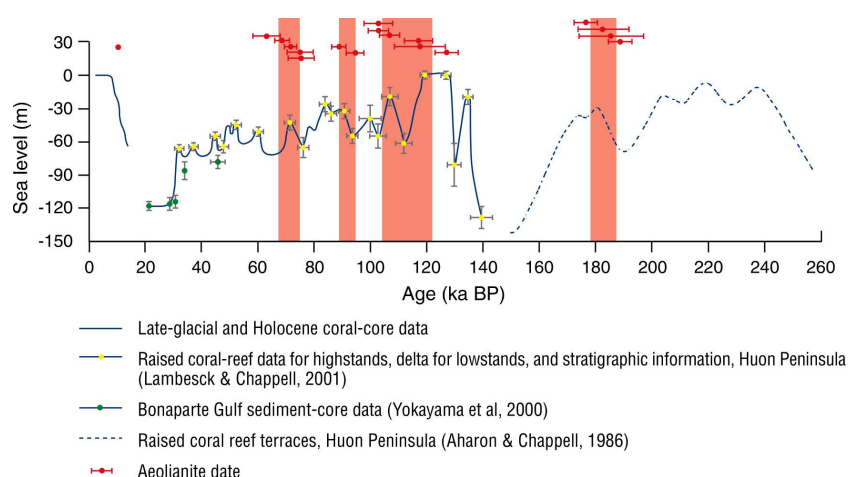
Fig. 9. Ages from aeolian sediments on the southern Cape, South Africa compared to the relative sea-level curve for the penultimate and last glacial cycle for the Huon Peninsula supplemented with observations from Bonaparte Gulf, Australia. Error bars define the upper and lower limits (modified from Lambeck et al. , 2002). Aeolianite age data are from Wilderness seaward cordon (this paper, Vogel et al. , 1999), Cape Agulhas aeolianites (this paper), Blombos Cave (Henshilwood et al. , 2002), Western Cape aeolianites (Roberts and Berger, 1997; Shaw et al. , 2001) and Eastern Cape aeolianite (Vogel et al. , 1999; Ramsay and Cooper, 2002). Shading relates to mean71 standard deviation of clusters of ages.
