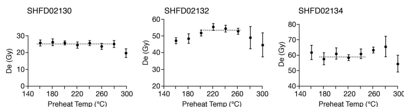
Fig. 7. Examples of preheat plateau tests undertaken to establish most appropriate preheat temperature to use in the SAR dose protocol for southern Cape samples. Note that measurements used only a reduced point SAR protocol. Separate data, with better characterised growth curves were generated for use in age calculations.
