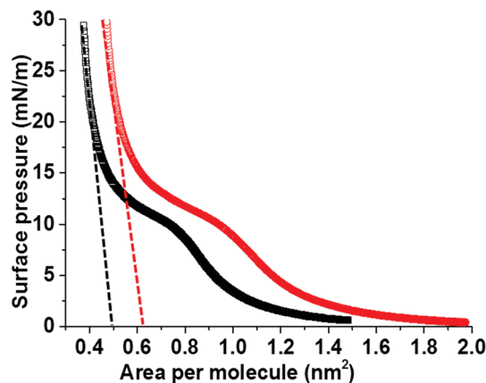
Fig. 7 Langmuir isotherms of DPPC + 5% DSPE-PEG 2000 monolayers, on water sub-phase (black) and water with 10 \mu L mL^{-1} C_6F_{14} added to the sub-phase (red). Dashed lines show the extrapolated average molecular area for the DPPC/DSPE-PEG 2000 phase.
