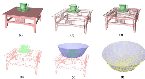
Fig. 2. Steps for computing IBS: Given a segmented scene (a) (in this example the scene have two segments: a cup and a table), which is composed of polygon meshes (b), we first subdivide the mesh to triangles of similar size (c) and then take the centre points of each triangle (d). IBS is the Voronoi surfaces which produced by two samples from different objects (e) and is also represented by a polygon mesh (f).
