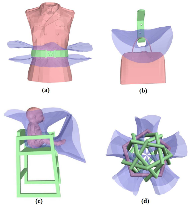
Fig. 1. Examples of the Interaction Bisector Surface (the blue surface) for two parts of the 3D scene (shown as red and green). (a) belt on uniform, (b) bag on hook, (c) baby on chair, (d) a pentagon tangled with other five pentagons
