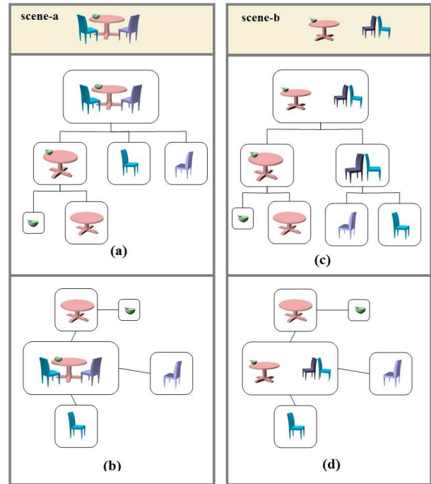
Fig. 6. Scene structures of two example scenes: scene-a and scene-b. (a) and (c) show the hierarchical structures produced by our method; (b) and (d) show the scene graph used in [Fisher et al. 2011].
