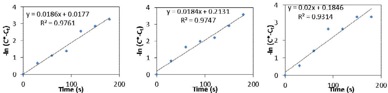
Figure 3: Plots of microbubble mass transfer rate against time at varying flowrate. Rate of oxygen transfer increased directly with increase in flow rate (Q). (a) Q = 0.1 L/min; k_{La} = 0.0161 Hz (b) Q = 0.3 L/min; k_{La} = 0.0171 Hz (c) Q = 0.5 L/min; k_{La} = 0.0186 Hz (d) Q = 0.7 L/min; k_{La} = 0.0184 Hz (e) Q = 0.9 L/min; k_{La} = 0.02 Hz. Dissolved O_2 level in the liquid medium increased continuously with time and reached saturation at 200 s.
