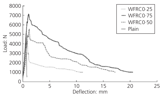
Figure 5. Flexural load–deflection curves of WFRC and plain specimens
