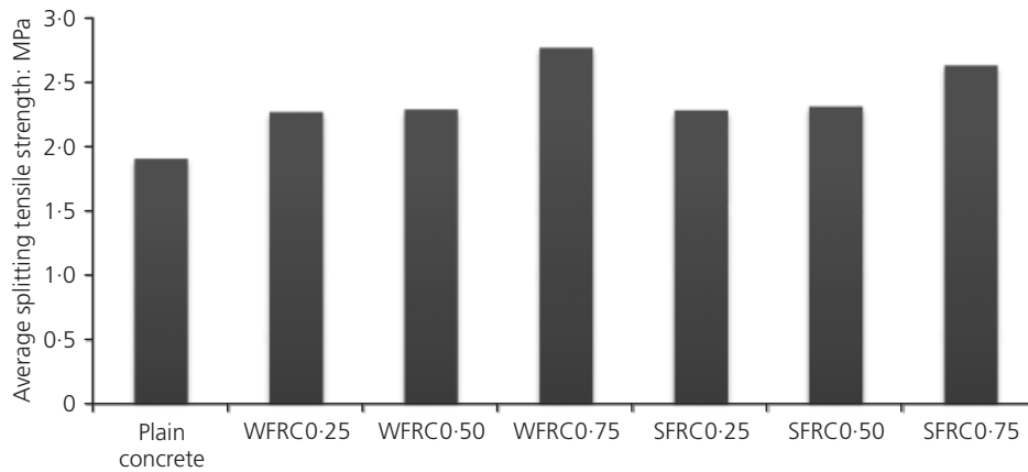
Figure 3. Average splitting tensile strength of WFRC, SFRC and plain specimens
