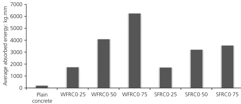
Figure 7. Average amount of absorbed energy by bending samples in kg.mm
