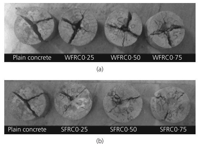
Figure 8. Comparison of failure patterns of FRC specimens after impact testing: (a) WFRC; (b) SFRC
