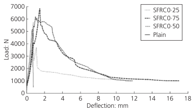
Figure 6. Flexural load–deflection curves of SFRC and plain specimens
