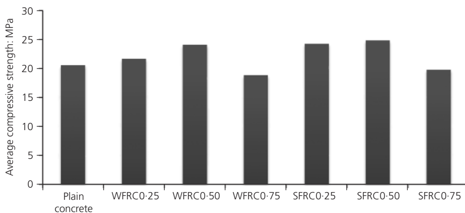
Figure 2. Average compressive strength of WFRC, SFRC and plain specimens
