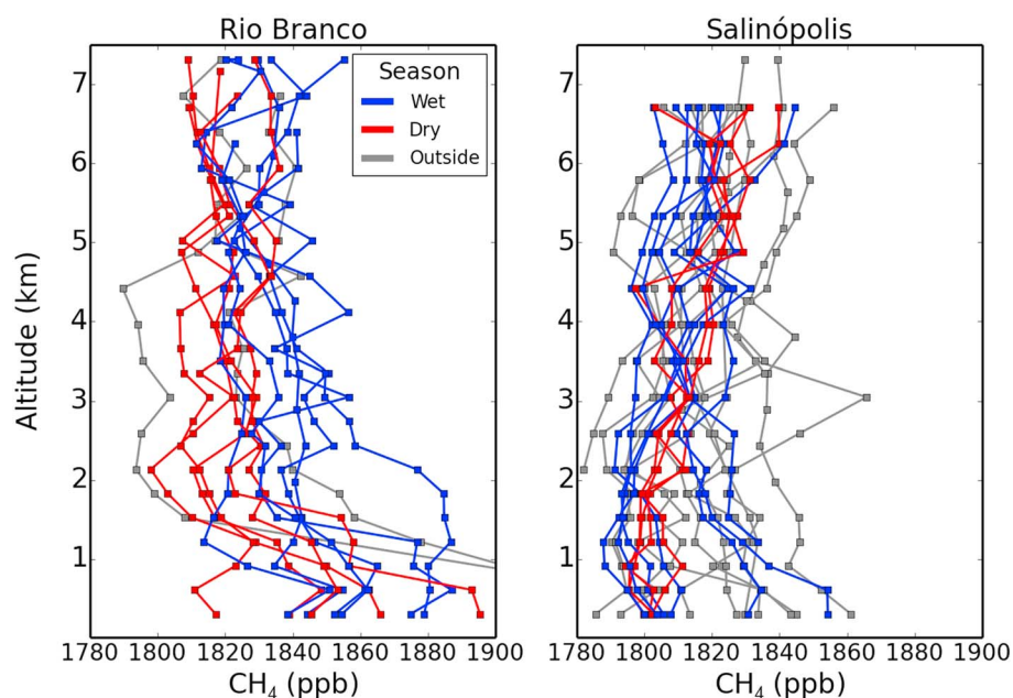
Figure 1. Amazonian Carbon Observatory aircraft measured \text{CH}_4 vertical concentration profiles taken between 2013 and June 2015 at Rio Branco and Salinópolis. Profiles measured between January–April are shown in blue, July–October in red, and May–June and November–December in gray.
