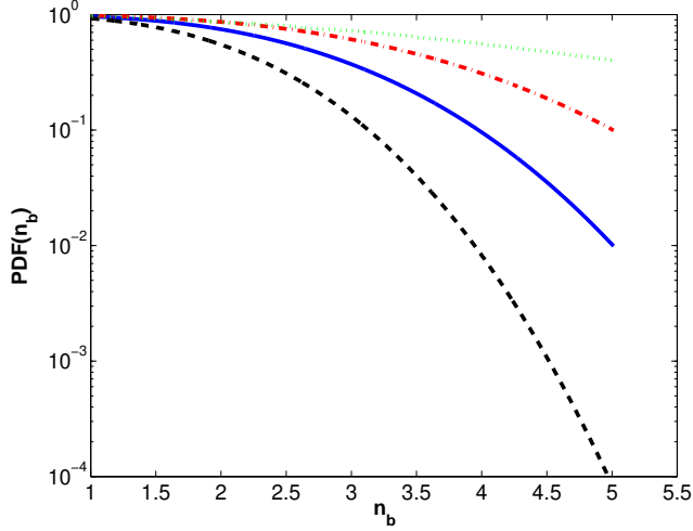
Figure 1: (Color online). The blob density PDF tail as a function of n_b normalized by N . The parameters are \gamma = \frac{K}{L_y^2 L_x \xi} = 0.33 (red line, dash-dotted), \gamma = 0.66 (blue line, solid line) and \gamma = 1.35 (black line, dashed line) with \kappa_0 = 6.0 . the Gaussian distribution (green line, dotted line) is shown with \gamma = 0.66 and \kappa_0 = 6.0 .
