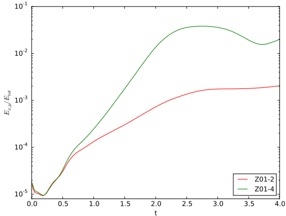
Figure 8. The ratio of magnetic energy in the x and y components over the total magnetic energy for two runs with initial conditions that of Z01-2 (red) Z01-4 (green) and a perturbing field containing 2 \times 10^{-5} of the total energy. The time is expressed in units of \tau_H .
