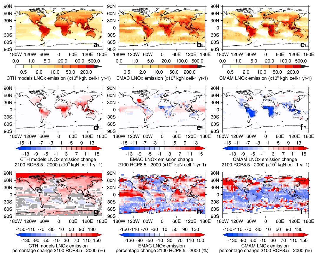
Figure 2. Annual vertically integrated lightning \text{NO}_x emission distribution for the year 2000 baseline, and absolute and percentage change with respect to RCP8.5 year 2100. Annual emissions for year 2000 distributions are normalized to 5 TgN for all models with the same normalization factors applied to year 2100 RCP8.5 emissions. Shown are (a–c) the baseline distributions for year 2000, (d–f) the absolute changes in distribution for the year 2100 RCP8.5 experiments, and (g–i) the equivalent percentage changes. The left column plots are the mean of eight models using the cloud top height approach. The middle and right column plots are the individual results for the EMAC and CMAM models, respectively. Mean values are calculated after scaling and regridding all models to a common resolution ( 5^\circ \times 5^\circ ). In Figure 2g the greyed cells represent grid cells in which there is not at least five models that estimate the same sign of change.
