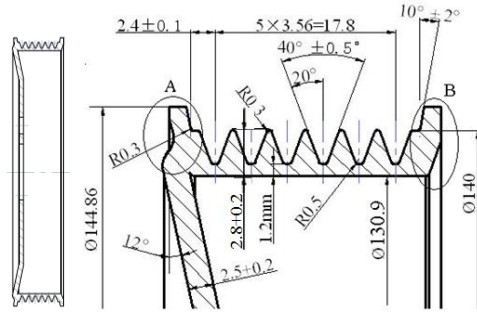
Fig. 22. Schematic of six-wedge poly-pulley [38].
