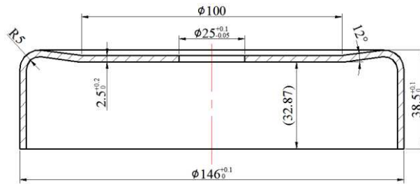
Fig. 23. Preforming drawing blank [38].
