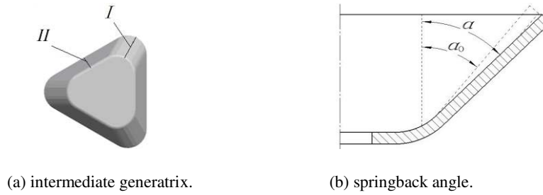
Fig. 44. Evaluation of geometrical accuracy [53].
