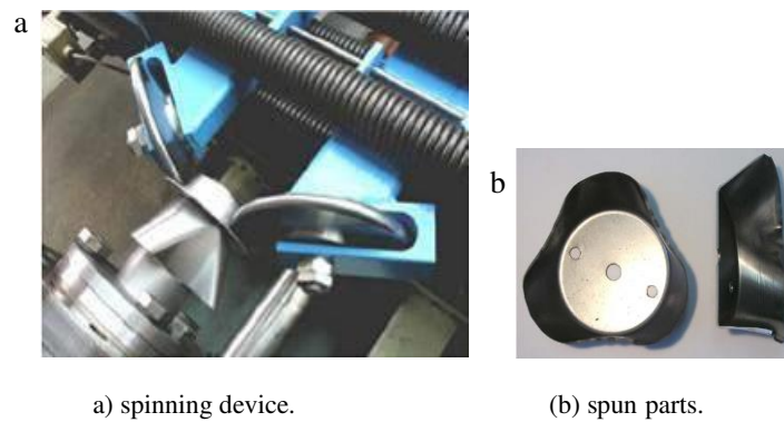
Fig. 38. Tripod shaped spinning device and spun parts [6].
