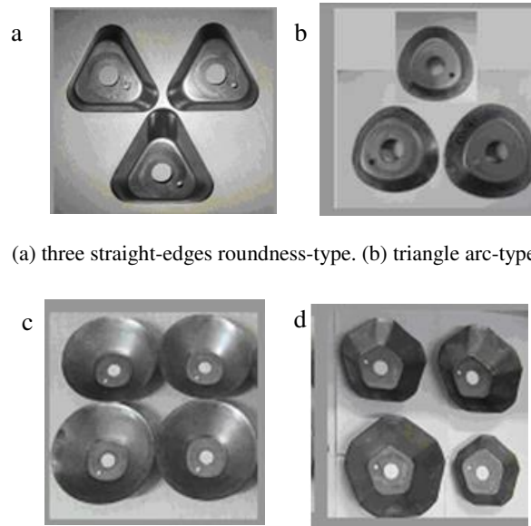
(c) quadrilateral arc-type. (d) five straight-edges roundness-type.
