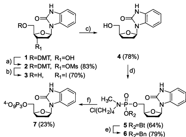
Scheme 1. Synthesis of 2',3'-dideoxy Benzi nucleotide. (a) MsCl, Pyr, 0°C. (b) (i) NaI, DME, 90°C; (ii) DCA. (c) H 2 , 10% Pd/C, MeOH. (d) (i) (4-chlorobutyl)(methyl)phosphoramidic dichloride, HOBT, THF, Pyr; (ii) NMI, THF. (e) BnOH, DMAP, THF. (f) (i) H 2 , 10% Pd/C, DMF; (ii) PPI.
