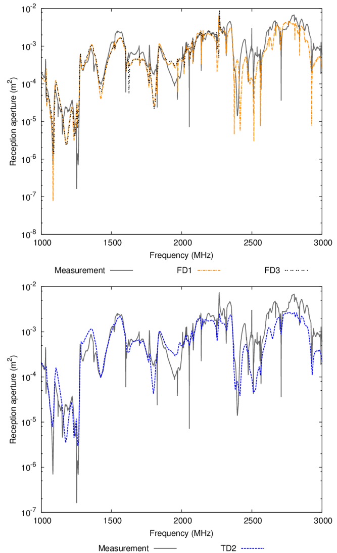
Fig. 11. Reception aperture for test case 1 from 1-3 GHz comparing frequency-domain codes (top) and time-domain codes (bottom) to measurement.
