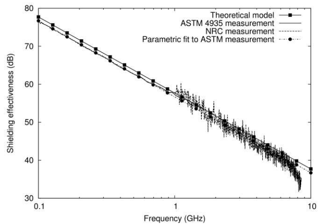
Fig. 5. Plane wave shielding effectiveness of an infinite perforated plate with the same characteristics as the front plate.
