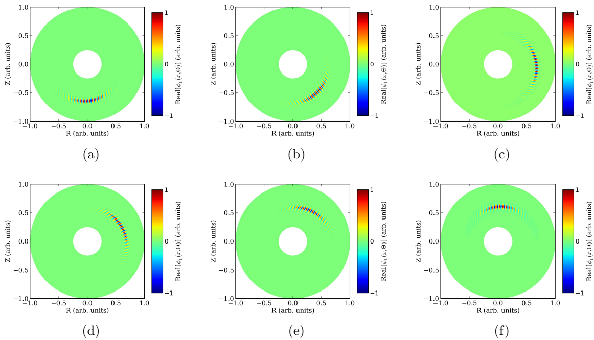
Figure 8: (Colour online) (a)-(f) show the poloidal mode-structure of the time evolving instability following a step in \gamma_E , with \gamma_E < \gamma_{E,\text{GM}} (chronologically at times indicated by arrows in Fig. 7c).
