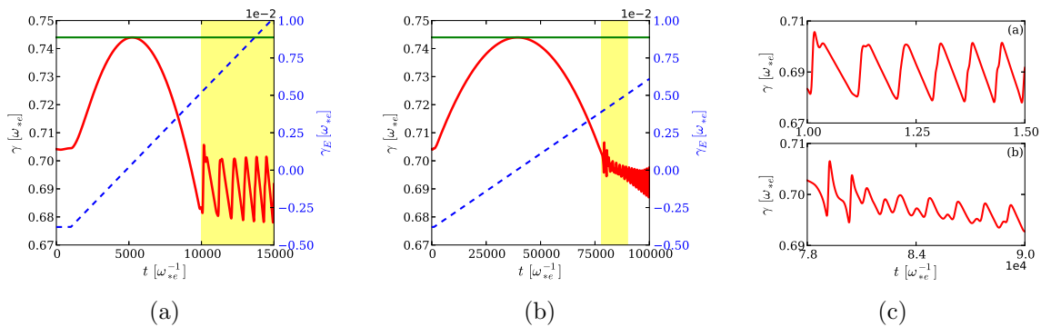
Figure 9: (a) shows the situation in Fig. 7a, except now the flow-shearing rate (dashed-blue line) has been pushed past \gamma_{E,\text{GM}} ; the case in (b) is for a much slower evolution of \gamma_E , with d\gamma_E/dt=1.0e-7 . Plot (c) shows the magnified images of the shaded regions in (a) and (b).
