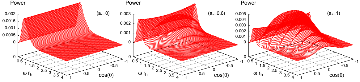
Figure 10: Angular distribution of the power spectra for emission of fermions on the brane from a rotating black hole, for n = 1 and a_* = (0, 0.6, 1) .
