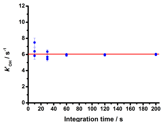
Figure 11. Observed OH reactivities, for a fixed gas composition (for which the expected OH reactivity is shown in red), as a function of averaging time, obtained using 15 mW of 308 nm probe laser power.
