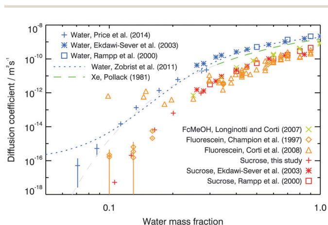
Fig. 9 Diffusion coefficients of water, 43,58,64,65 sucrose, 64,65 fluorescein, 39,41 ferrocene methanol 75 and xenon 25 in aqueous sucrose. Colour corresponds approximately to the size of the diffusant: the largest, sucrose, is shown in red, followed by fluorescein in orange, then ferrocene methanol in yellow-green, xenon in blue-green and finally water, the smallest, shown in blue. Water activities used in this study and reported by Zobrist et al. 43 and Price et al. 58 are converted to water mass fraction using the parameterisation given by Norrish. 66 The grey dashed line represents an extrapolation of the Pollack 25 parameterisation. We include this more speculative regime on the basis that the parameterisation is arrived at via a straight line fit in \log(\text{diffusion coefficient}) vs. \log(\text{viscosity}) space; the agreement with the Price et al. 58 water diffusion coefficient data is interesting.
