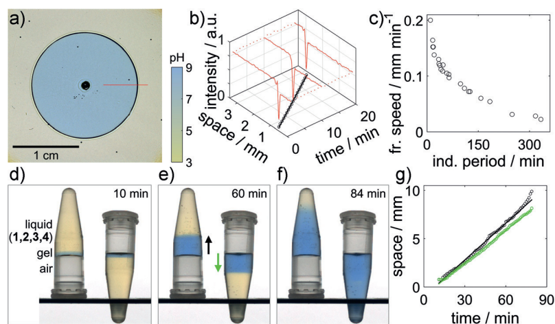
Figure 3. Frontal polymerization. Experiments with a pH indicator (bromothymol blue) in a) a thin layer in a petri dish and d–g) two 4 mL vials with identical reaction mixtures. Fronts were initiated with NaOH (pH 8). a) Image taken by shadowgraphy (see the Supporting Information) showing the position of the polymerization front (dark band) and the pH front (yellow to blue). b) Intensity profiles along a slice (red line in (a)) in images at three different times (high intensity: yellow; low intensity: blue; spike: dark band) and position of the front with time (circles with a straight-line fit). c) Front speed in the petri dish as a function of the induction period in a well-stirred mixture. d–f) Images of ascending and descending fronts. g) Front position as a function of time (black: ascending fronts; green: descending fronts). Component concentrations: [ETTMP] 0 = 0.17 M, [PEGDA] 0 = 0.24 M, [urease] = 29 units mL −1 ; T = 20 °C; [urea] = 0.11 (a,b), 0.04–0.27 (c), 0.09 M (d).
