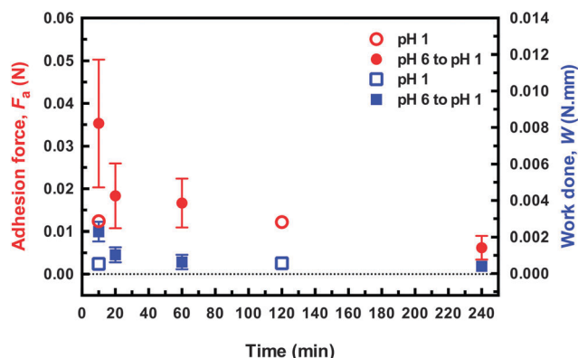
Fig. 5 Adhesion force and work done in removing the DN hydrogel probe from the brush surface for different times after immersion in pH 1 solution for samples that were either brought into contact at pH 1 or pH 6. The applied force in both cases was 0.1 N, and was applied 2 min. The force–distance curves for these data are shown in the ESI.†
