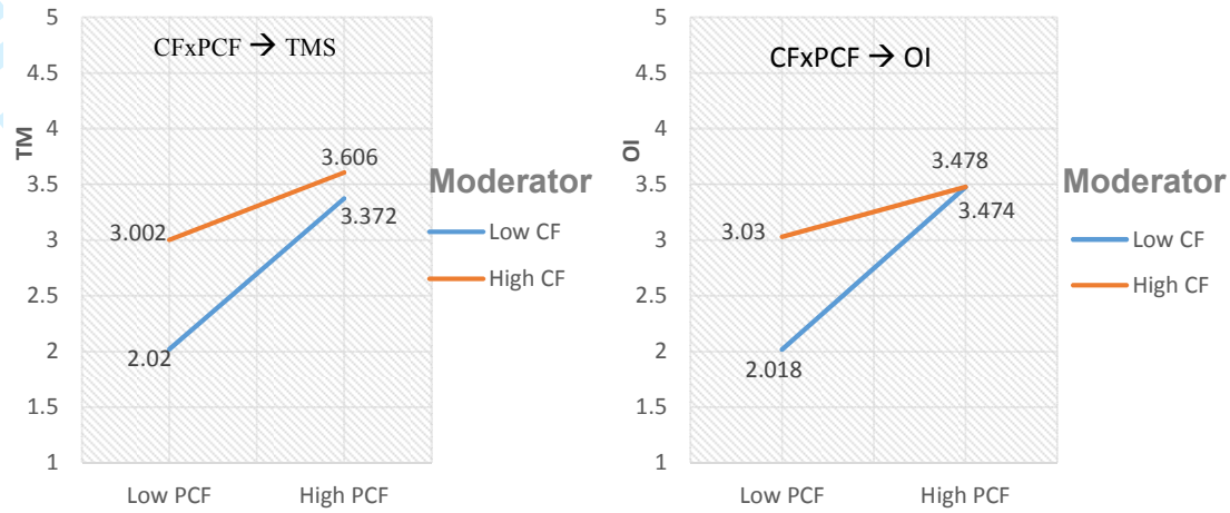
Figure 2: Interaction effect of the product variable - (CF x PCF) on Organizational Interoperability and Transactive Memory Systems
