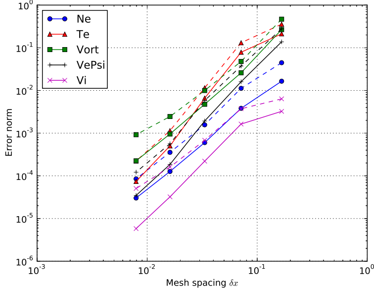
FIG. 11. Error norms for 5-field set of equations. Solid lines show the l^2 (RMS) error norms, whilst dashed lines are the l^\infty (maximum) error. Convergence orders for density N_e is 2.02; electron temperature T_e is 2.70; Vorticity \omega is 2.04; Electron parallel velocity V_e is 2.36; and ion velocity V_i is 2.42. Resolutions range from 8^3 to 128^3 . Script: examples/MMS/GBS/runtest-slab3d
