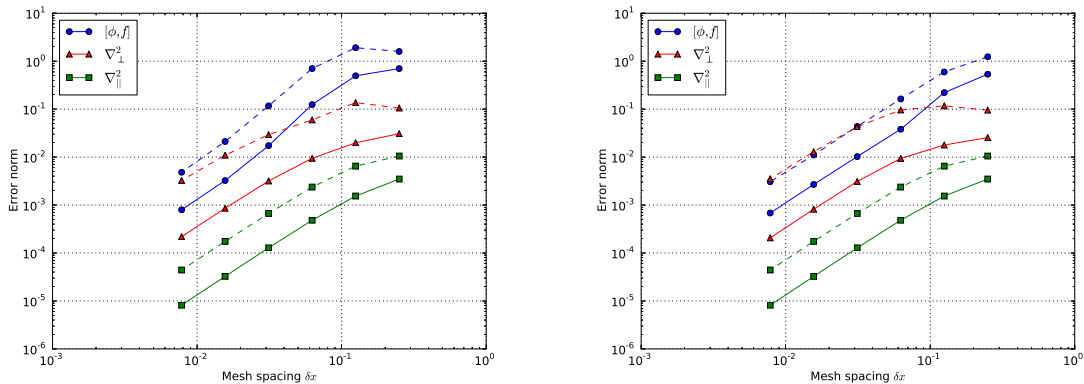
(a)Ballooning coordinates. Convergence rates for Arakawa bracket (2.03); perpendicular diffusion operator (1.97); and parallel diffusion operator (1.99) (b)Shifted metric method. Convergence rates for Arakawa bracket (2.07); perpendicular diffusion operator (1.98); and parallel diffusion operator (1.99)
