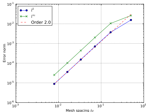
FIG. 4. Error norms for f in wave equation 15 using 2^{nd} -order central differencing. A convergence rate of 1.97 is found, illustrated with a dashed line. Script:examples/MMS/wave-1d/runtest
