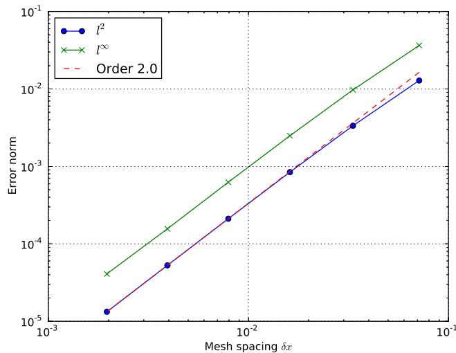
FIG. 9. Error norm of Hasegawa-Wakatani system ( n and \phi , equations 25) on a Cartesian mesh, showing second-order convergence. Mesh resolutions range from 16 \times 16 to 512 \times 512 .
