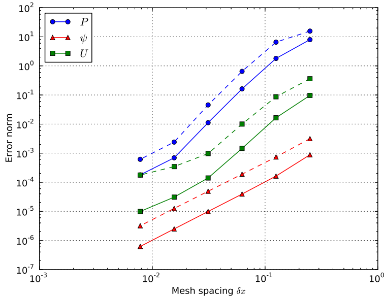
FIG. 10. Error norms for 3-field set of equations. Solid lines show the l^2 (RMS) error norms, whilst dashed lines are the l^\infty (maximum) error. Convergence orders for pressure p is 1.95; vorticity \omega is 1.64; and vector potential A_{||} is 2.01. Resolutions range from 4^3 to 128^3 . Script: examples/MMS/elm-pb/runtest
