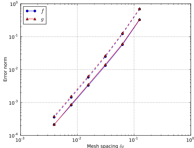
FIG. 8. Convergence of f (1.95) and g (2.04) in equation 15 solved using the FCI method in a sheared slab. Solid lines show l^2 (RMS) error, whilst dashed lines show l^\infty (maximum) error. Script:examples/fci-slab/runtest
