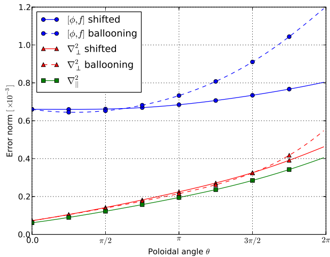
FIG. 7. Comparison of RMS error norm for ballooning (dashed lines) and shifted-metric scheme (solid lines), as function of poloidal angle \theta , for the highest resolution case in figure 6 ( 128^3 grid points). Integrated shear I (equation 10) is zero at \theta = 0 , and a maximum at \theta = 2\pi .
