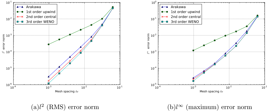
FIG. 3. MMS test of advection operators. Equation 12 is solved on a 2D domain with uniform grid spacing. The resolution varies from 16 \times 16 to 1024 \times 1024 . Convergence rates for second-order Arakawa (1.998), 1 st -order upwind (0.993), 2 nd -order central differencing (2.005), and 3 rd -order WENO (2.019). All methods are limited to at best second-order in mesh spacing \delta x due to the central differencing applied to \phi and the boundary conditions. Script:examples/MMS/advection/runtest
