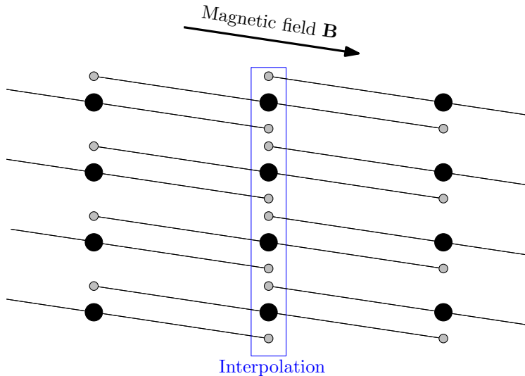
FIG. 1. Flux Coordinate Independent (FCI) scheme. To calculate the derivative along the magnetic field at grid cells (large solid circles), field-lines are followed in both directions to points on neighbouring planes of grid cells (small open circles). Values at these points are found by high-order interpolation using nearby points (blue box).
