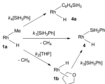
Scheme 3. Kinetic Analysis of Reactivity of 1a
