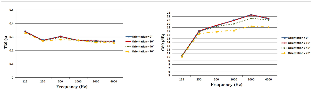
Figure 4. Comparing T30 and C80 values observed from a single receiver point in a virtual shoebox model by varying the orientation of the virtual Genelec S30D sound source (0° to 10°, 40° and 70°).
