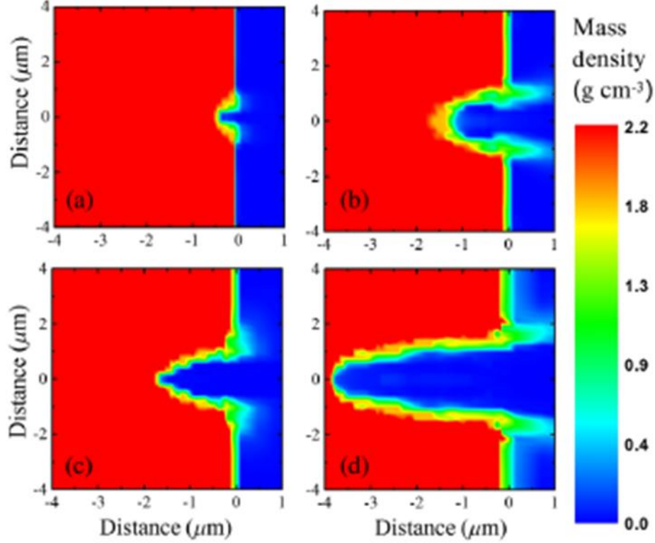
Figure 1. Single shot ablation profiles of craters in parylene-N irradiated by an EUV (wavelength 46.9 nm) laser of 1.3n pulse duration at different peak irradiances (a) 10^9 \text{ W cm}^{-2} , (b) 10^{10} \text{ W cm}^{-2} , (c) 10^{11} \text{ W cm}^{-2} and (d) 10^{12} \text{ W cm}^{-2} . The focal spot diameter assumed is 500 nm (originally published by Rossall et al 7 ).
