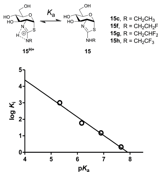
Fig. 5 Acid dissociation of the 2'-aminothiazolium protonation state of 2'-aminothiazoline inhibitors 15c and 15f–h and the linear free energy relationship (LFER) analysis between the \text{pK}_a and \log K_i . Of these inhibitors shows a negative correlation of -1.12 \pm 0.09 .
