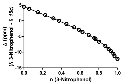
Fig. 4 A representative example for ^{13}\text{C} -NMR determination of the \text{pK}_a value for ThiamEt-G ( 15c ) with chemical shifts of the 2'-C of the thiazoline ring resonances ( \Delta ppm) for compounds 15c as a function of the fractional protonation ( n ) of the reference compound, 3-nitrophenol ( \text{pK}_a of 8.42). The solid line is the best non-linear least squares fit to eqn (S1) (ESI†).
