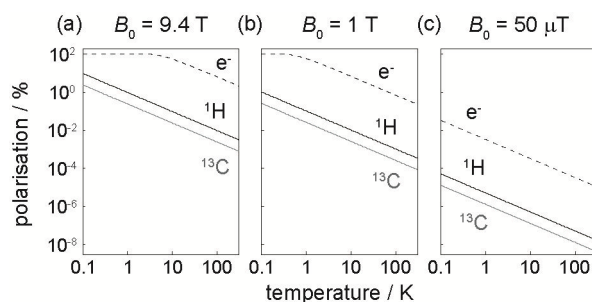
Figure 1. Polarisation level as a function temperature for ^{13}\text{C} nuclei (grey lines), ^1\text{H} nuclei (black lines) and unpaired electrons (dashed lines) with (a) B_0 = 9.4\text{ T} , (b) B_0 = 1\text{ T} , and (c) B_0 = 50\text{ }\mu\text{T} .
