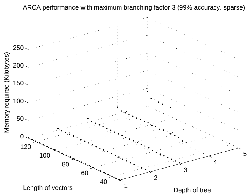
Fig. 8 Scatter plots showing the recall performance for ARCA where the branching factor is 3, with a target of 99% accuracy. At the top is the memory required when storing CMMs explicitly using MATLAB, and at the bottom is the memory required when storing CMMs using the binary Yale format in ENAMeL. Each point represents a successful recall in at least 99 of the 100 experimental runs.
