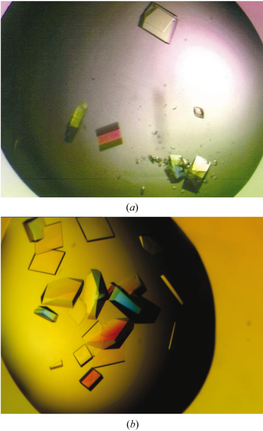
Figure 1 (a) Monoclinic (form II) crystals of Pre-N175A precursor and (b) (form I) crystals of N175A mutant proteins of B. sphaericus PVA.
