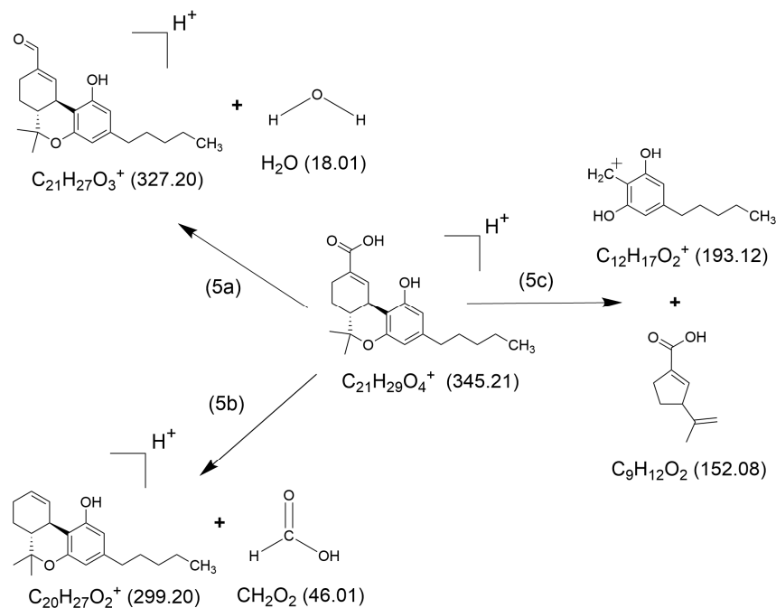
Figure 5. Suggested structures of the major ionic fragments and their neutral counter-fragments (5a)–(5c) observed in HCD experiment of [\text{THCOOH} + \text{H}]^+ . (Exact masses are given in parentheses).
