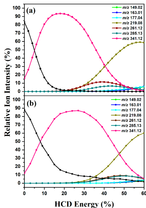
Figure 6. Precursor ion dissociation profile displayed with fragment ion production curves for (a) [\text{CBDA} + \text{H}]^+ ( m/z 359.18) and (b) [\text{THCA} + \text{H}]^+ ( m/z 359.18) displayed as a function of HCD energy. The solid line is a three-point adjacent average of the data points. The black line corresponds to the precursor ion.
