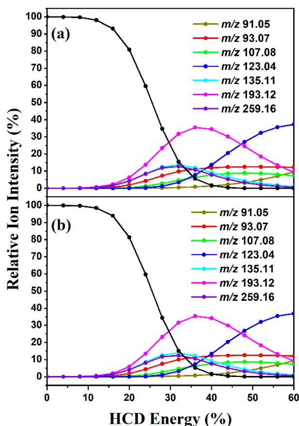
Figure 1. Precursor ion dissociation curve along with fragment ion production curves for (a) [\text{CBD} + \text{H}]^+ ( m/z 315.23) and (b) [\text{THC} + \text{H}]^+ ( m/z 315.23) displayed as a function of HCD energy. The solid line is a three-point adjacent average of the data points (the black line corresponds to the precursor ion).
