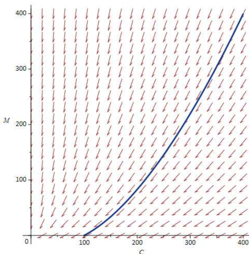
Fig. 1. Phase portrait of Civilian C and Militant M numbers under the model with \beta = \frac{1}{3} (and \alpha = 10 , which does not affect the plot). Trajectory is from C_0 = 400 , M_0 = 400 and terminates at C = 100 , M = 0
