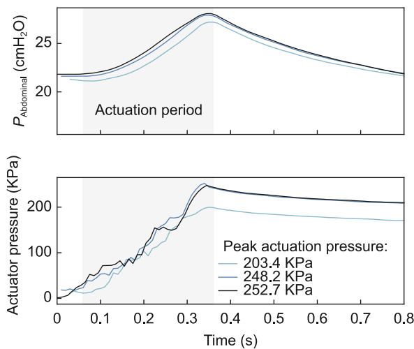
Fig. 4. The abdominal pressure (above) and the actuator pressure (below) throughout the ventilation cycle. Between 0.05 and 0.34 s the actuators are pressurised and push on the diaphragm, causing the abdominal pressure to increase. After reaching a set pressure the actuators depressurise returning the system to its normal pressure. This was done at peak actuation pressures of 203.4 KPa, 248.2 KPa, and 252.7 KPa.
