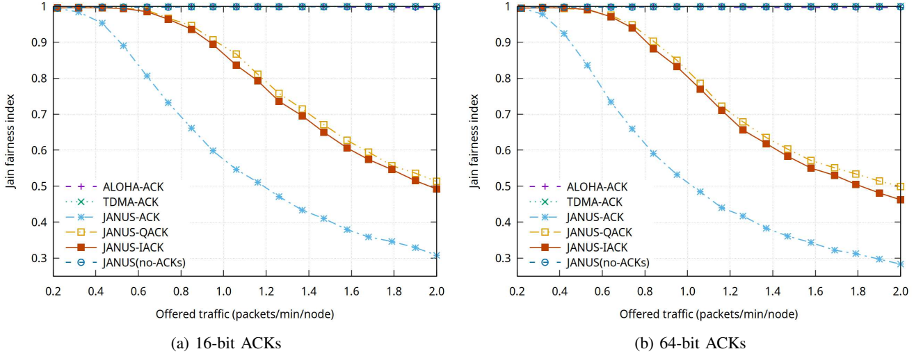
Fig. 8: Jain's fairness index (15 hours of simulated time)
