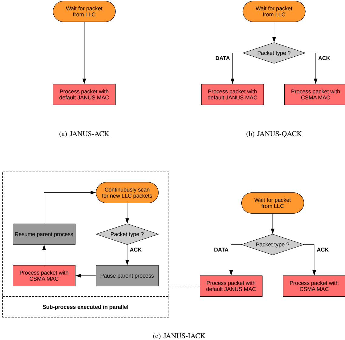
Fig. 4: Representation of the different ACK integration strategies implemented in the three JANUS variants
