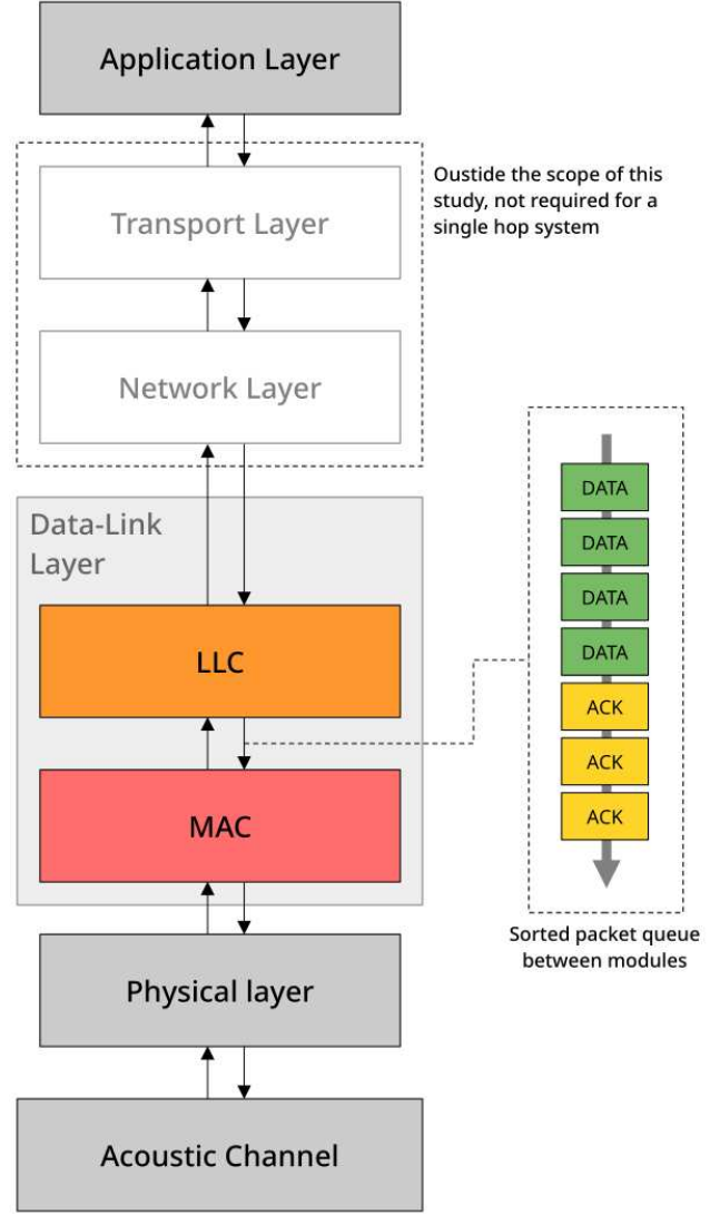
Fig. 3: Representation of the implemented network stack in this study. On the right is a representation of the packet queue present between each layer and sub-layer
